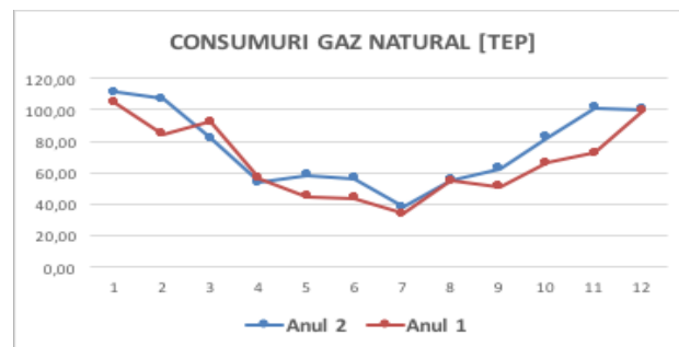
Fig. 7. Consumuri energetice lunare
