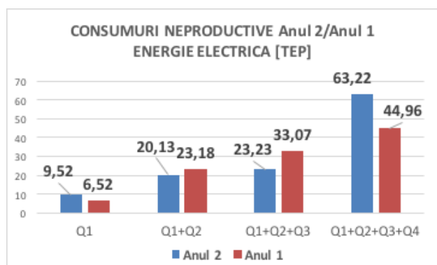
Fig. 13. Consumuri energetice neproductive anuale
