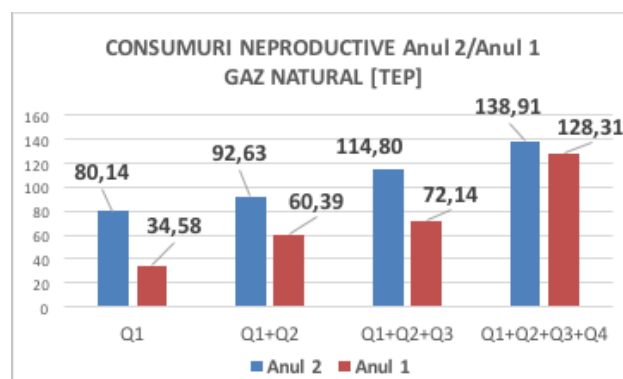
Fig. 13. Consumuri energetice neproductive anuale
